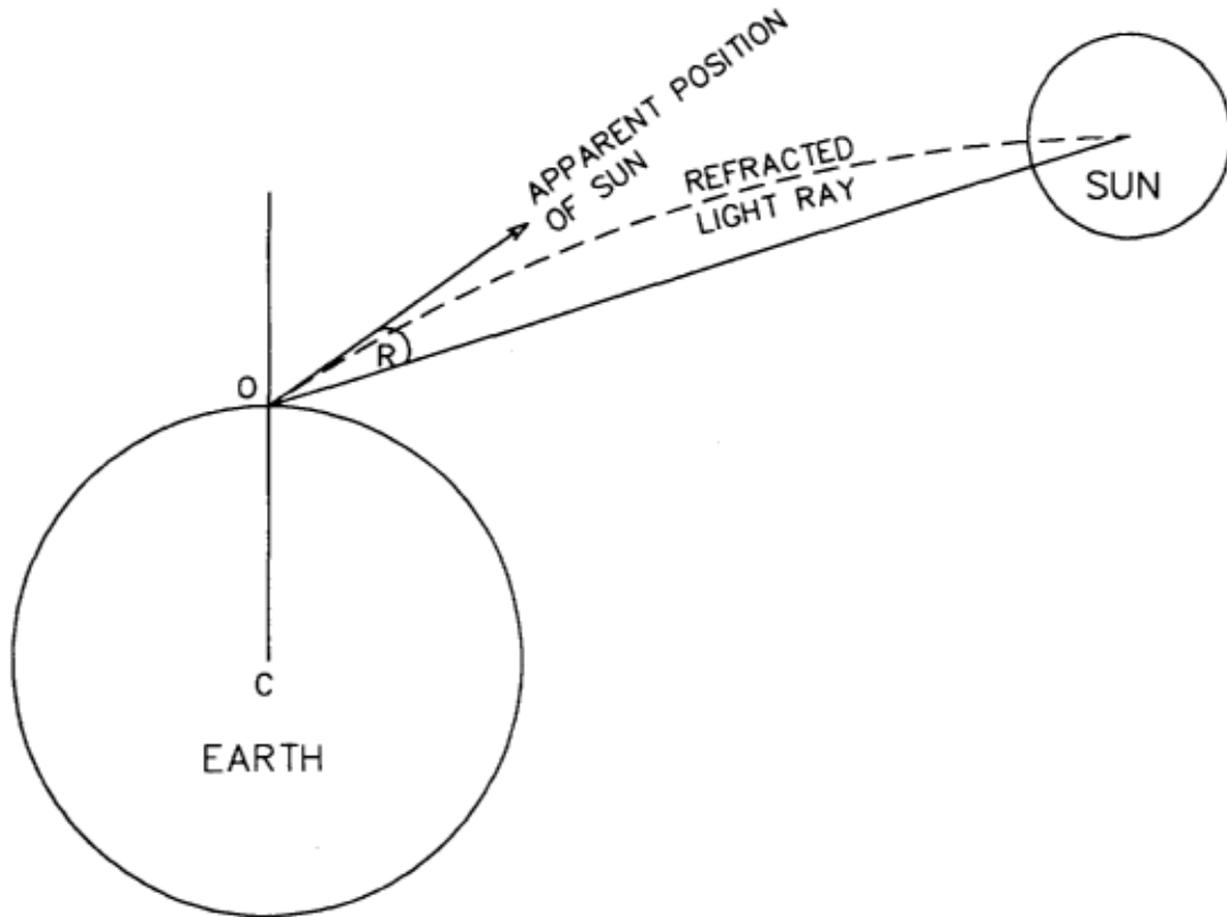
Figure 7. Refraction correction.
