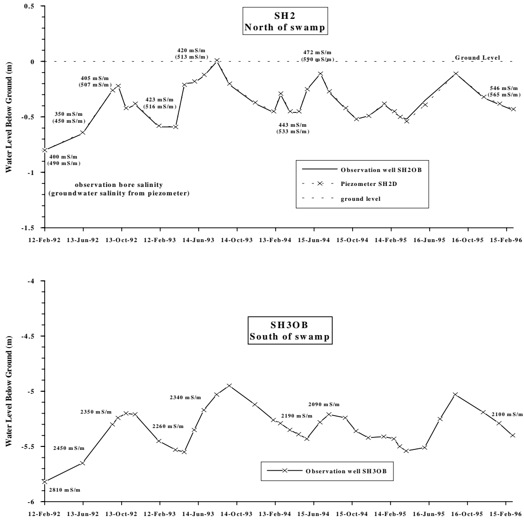
Figure 2. Hydrographs for groundwater monitoring sites.
